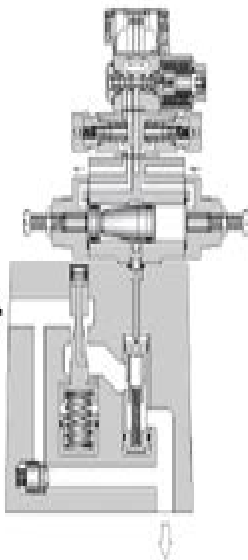
Pilot Operated Flow Control Valve
