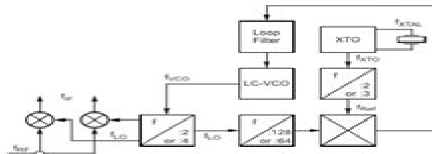
Figure 1. System Block Diagram for the Receivers Containing the Internal Frequency Generation and Processing (Synthesizer)
