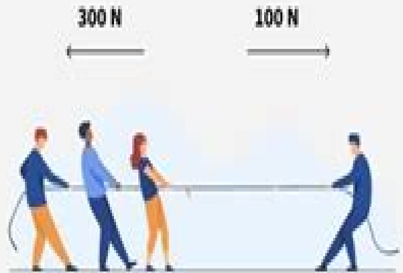
Unbalanced forces
