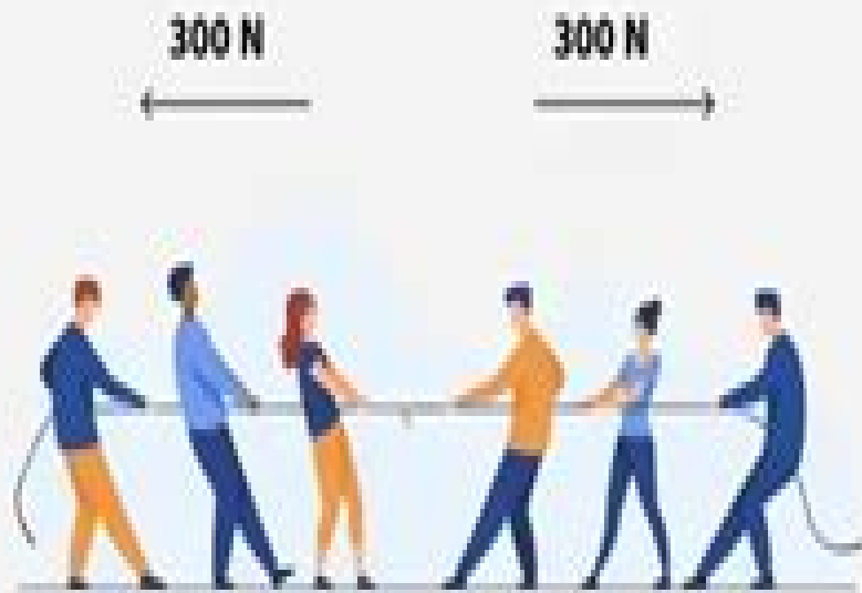
Balanced forces
