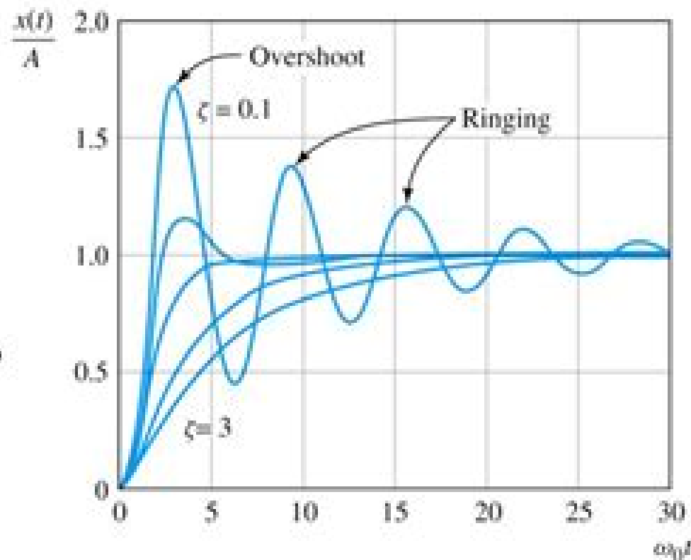
Figure 4.29 Normalized step responses for second-order systems described by Equation 4.99 with damping ratios of \zeta = 0.1, 0.5, 1, 2 , and 3 . The initial conditions are assumed to be x(0) = 0 and x'(0) = 0 .
