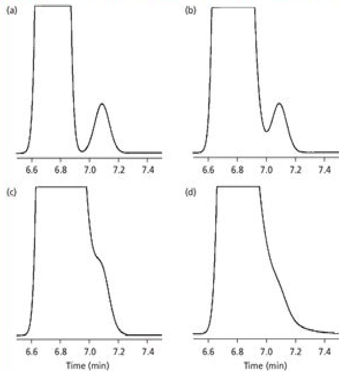
Figure 3: Same as Figure 2, except the peak area ratio for the two peaks is 100:1.
