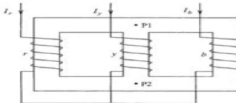
Figure 2.7 Three-phase three-limb core with Y connected primary
