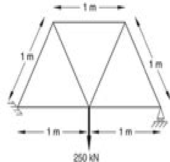
Figure 1. Schematic of an overhead hoist.
