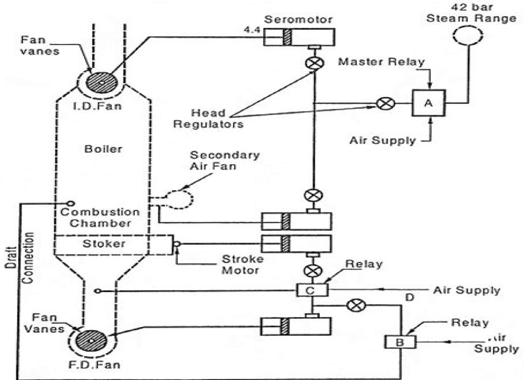
Fig: 5.21 Automatic Combustion Control System
