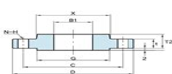
SLIP-ON
