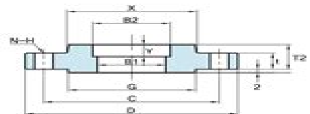
SOCKET WELDING
