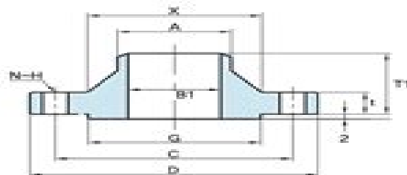
WELDING NECK
