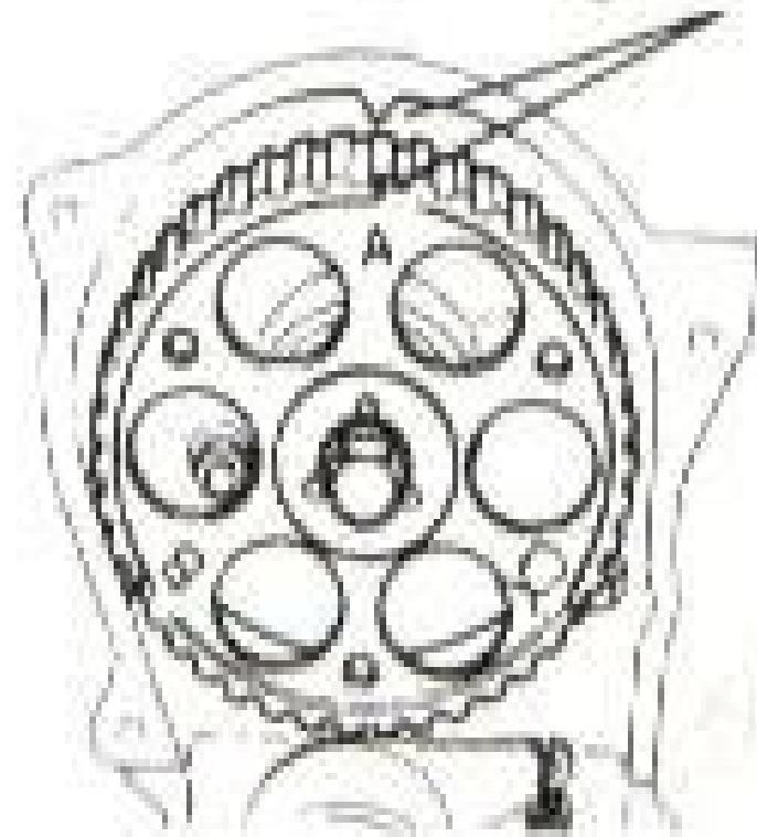
Timing mark
